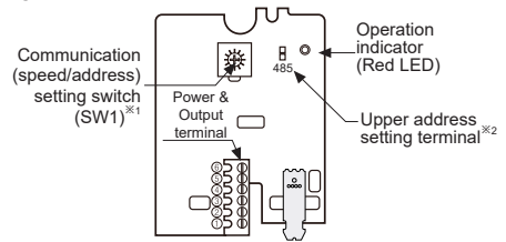
<Inner PCB of THD-D/THD-W>
